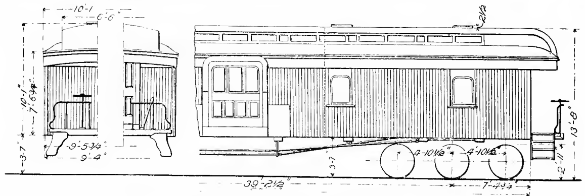
Figs. 168-170. REFRIGERATOR EXPRESS CAR. BALTIMORE & OHIO RAILROAD.
